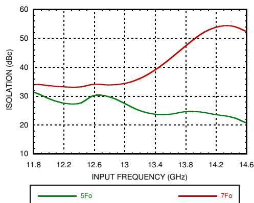
5th & 7th Harmonic Isolation, Pin = 4dBm VD_MULT = +1.5V, VD_AMP = +4V
