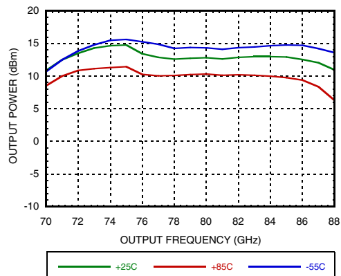
Output Power vs. Temperature [1]
