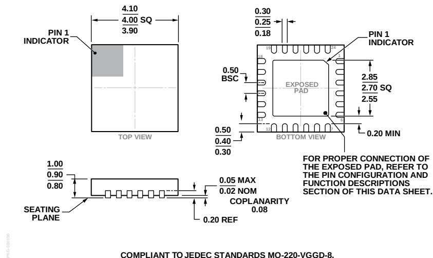
Figure 27. 24-Lead Lead Frame Chip Scale Package [LFCSP] 4 mm × 4 mm Body and 0.90 mm Package Height (CP-24-16) Dimensions shown in millimeters
