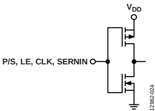
Figure 6. P/S, LE, CLK, and SERNIN Interface
