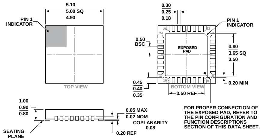
Figure 17. 32-Lead Lead Frame Chip Scale Package [LFCSP_VQ] 5 mm × 5 mm Body, Very Thin Quad (HCP-32-1) Dimensions shown in millimeters
