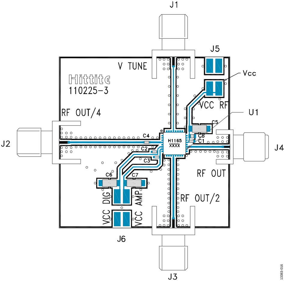
Figure 17. Evaluation Board
