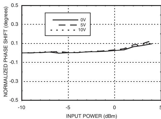
Phase Shift vs. Pin @ 18 GHz
