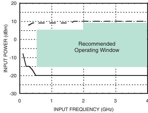
Input Sensitivity Window, T = 25^\circ\text{C}
