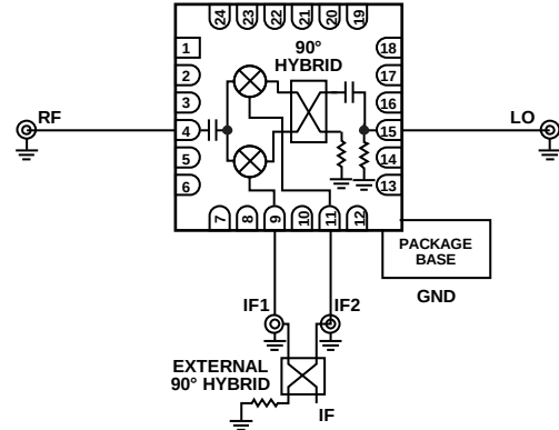
Figure 83. Typical Application Circuit
