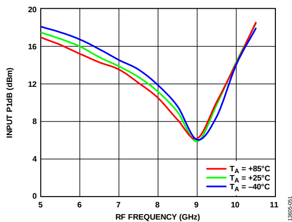
Figure 51. Input P1dB vs. RF Frequency at Various Temperatures
