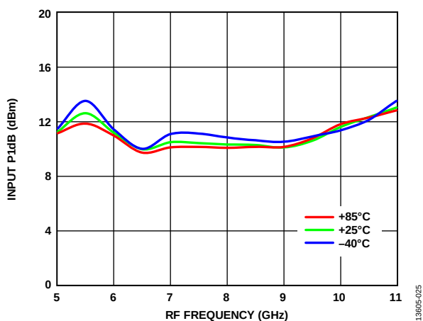
Figure 25. Input P1dB vs. RF Frequency at Various Temperatures
