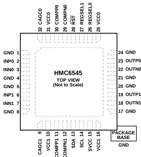
Figure 2. Pin Configuration
