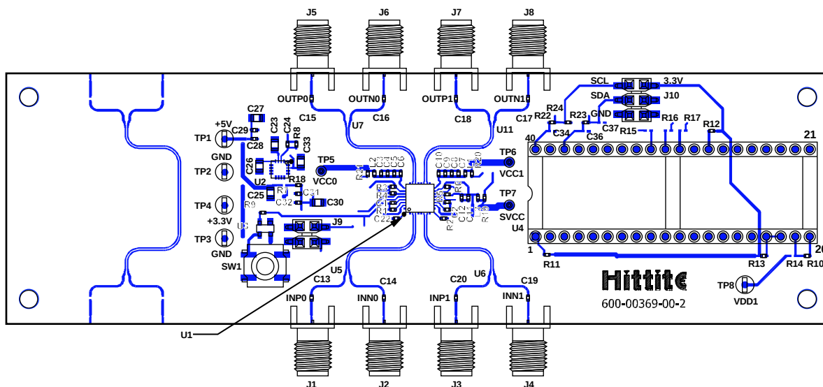
Figure 34. PCB
