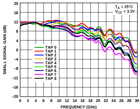
Figure 18. Small Signal Gain Over Taps, for S21 Line of Each Tap, Relevant Tap Is Set to Maximum Gain While Remaining Taps Are Enabled with No Gain
