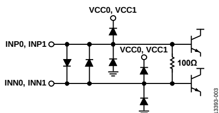
Figure 4. INPx, INNx Interface Schematic
