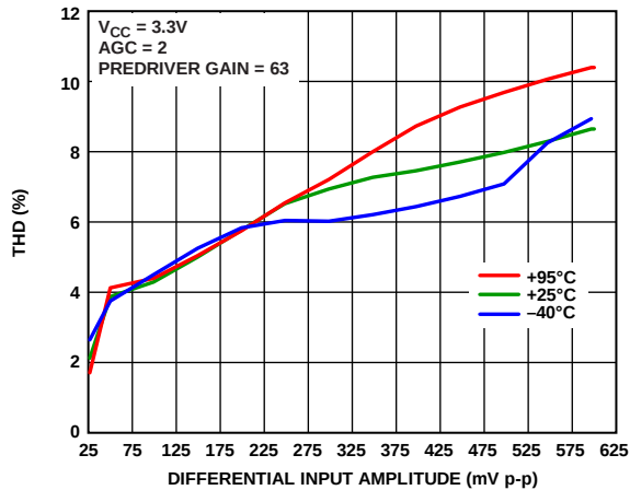
Figure 16. THD vs. Differential Input Amplitude Over Temperature, Tap 4 Gain Is Set to Maximum Gain, While Others Are Enabled with No Gain
