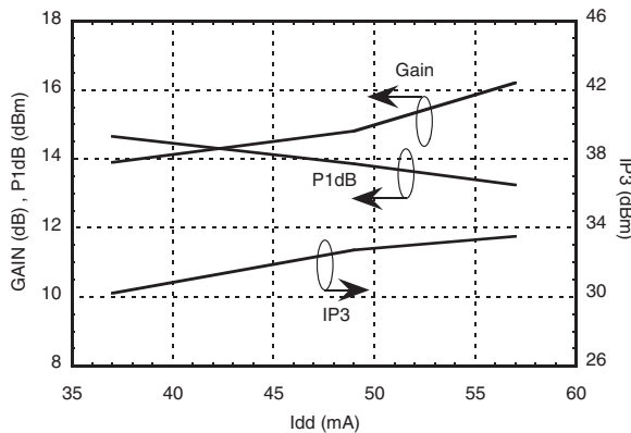
LNA - Gain, P1dB, Output IP3 vs. Current [1] @ 900 MHz
