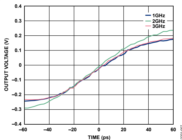
Figure 7. LVPECL Differential Output Voltage, 86 \Omega , 2.5 V vs. Carrier Frequency over Time, 2 dBm Input, Uncorrected for Board Loss, and Measurement Band Limited by the Trace Bandwidth
