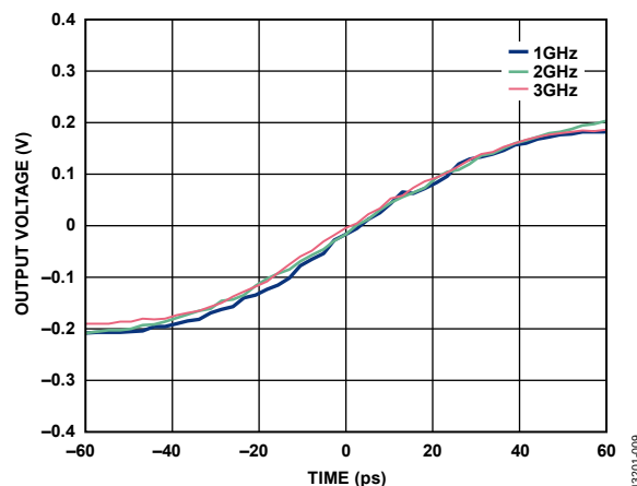
Figure 9. LVDS Differential Output Voltage, 100 \Omega , 2.5 V vs. Carrier Frequency over Time, 2 dBm Input, Uncorrected for Board Loss, and Measurement Band Limited by the Trace Bandwidth
