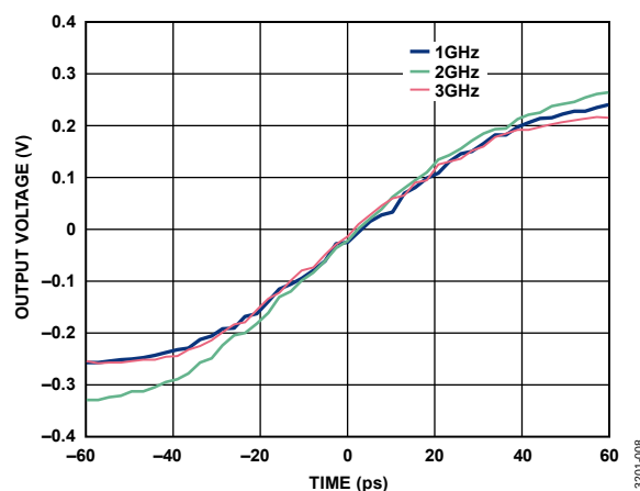
Figure 8. LVPECL Differential Output Voltage, 150 \Omega , 3.3 V vs. Carrier Frequency over Time, 2 dBm Input, Uncorrected for Board Loss, and Measurement Band Limited by the Trace Bandwidth
