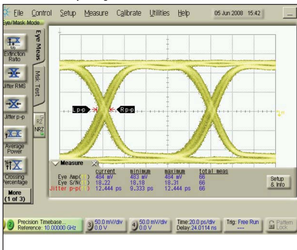
Eye Diagram [4]
