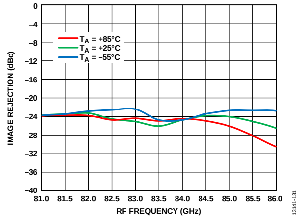
Figure 123. Image Rejection vs. RF Frequency at Various Temperatures, R_{FIN} = -20 dBm, LO = 2 dBm, IF = 500 MHz, V_{DLNA} = 3 V
