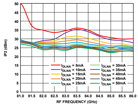
Figure 137. Input IP2 vs. RF Frequency at Various I_{DLNA} Values, R_{FIN} = -20 dBm, LO = 2 dBm, IF = 500 MHz, V_{DLNA} = 3 V
