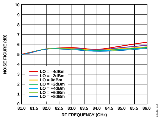
Figure 195. Noise Figure vs. RF Frequency at Various LO Powers, IF = 500 MHz, V_{DLN} = 3 V
