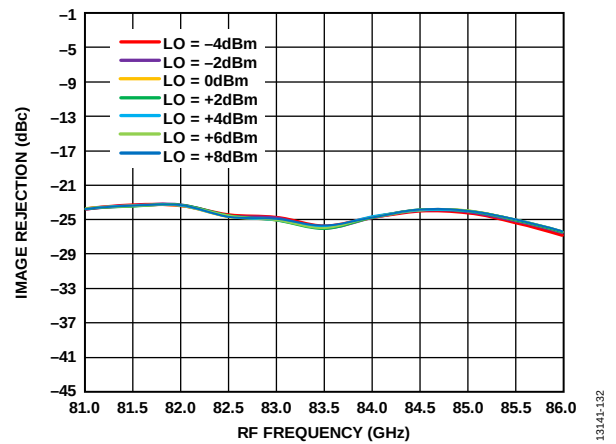
Figure 124. Image Rejection vs. RF Frequency at Various LO Powers, R_{FIN} = -20 dBm, IF = 500 MHz, V_{DLNA} = 3 V
