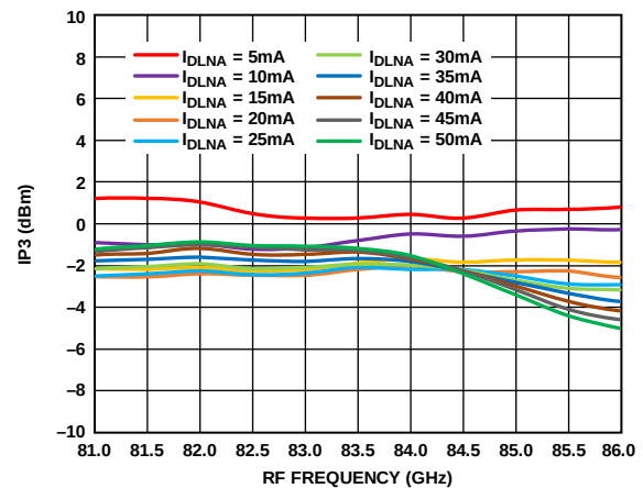
Figure 183. Input IP3 vs. RF Frequency at Various I_{DLNA} Values, R_{FIN} = -20 dBm, LO = 2 dBm, IF = 2000 MHz, V_{DLNA} = 3 V
