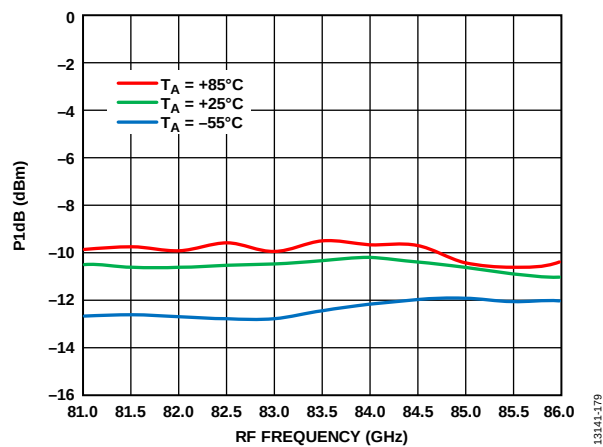
Figure 165. Input P1dB vs. RF Frequency at Various Temperatures, LO = 2 dBm, IF = 1000 MHz, V_{DLN} = 3 V
