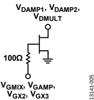
Figure 5. V GMIX , V DAMP1 , V DAMP2 , V DMULT , V VGAMP , V VGX2 , and V VGX3 Interface
