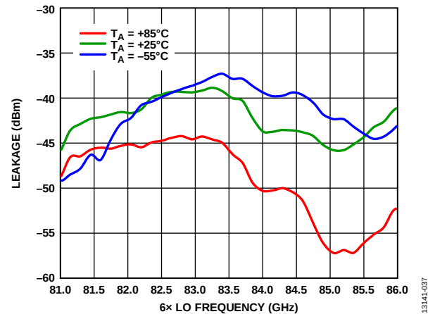
Figure 37. 6x LO Leakage at RFIN vs. 6x LO Frequency at Various Temperatures, LO = 2 dBm, V_{DLNA} = 3 V
