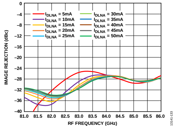
Figure 125. Image Rejection vs. RF Frequency at Various I_{DLNA} Values, R_{FIN} = -20 dBm, LO = 2 dBm, IF = 500 MHz, V_{DLNA} = 3 V
