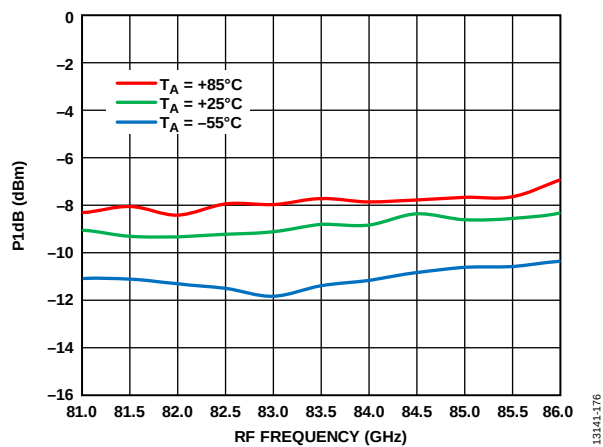
Figure 164. Input P1dB vs. RF Frequency at Various Temperatures, LO = 2 dBm, IF = 1000 MHz, V_{DLN} = 4 V
