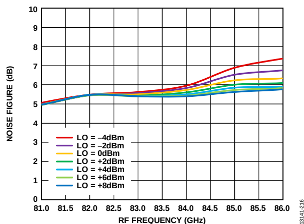
Figure 196. Noise Figure vs. RF Frequency at Various LO Powers, R_{FIN} = -20 dBm, IF = 500 MHz, V_{DLN} = 3 V
