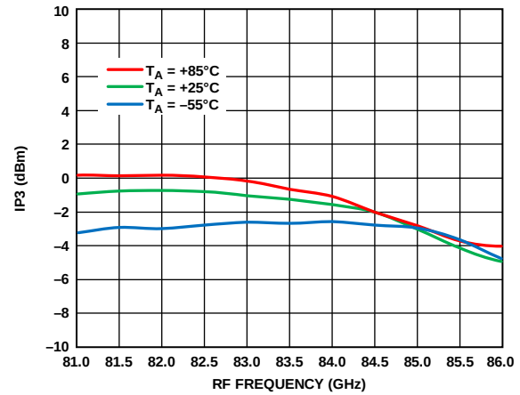
Figure 181. Input IP3 vs. RF Frequency at Various Temperatures, R_{FIN} = -20 dBm, LO = 2 dBm, IF = 2000 MHz, V_{DLNA} = 3 V
