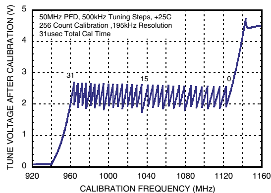
Typical VCO Tuning Voltage After Calibration
