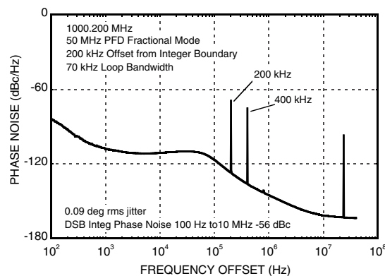
Typical Spurious at 200 kHz from Integer Boundary [1]
