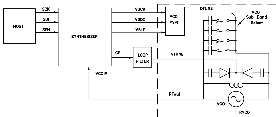
Figure 32. Simplified Step Tuned VCO
