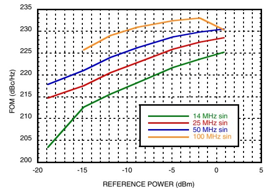
Figure 12. Reference Input Sensitivity Sinusoidal Wave, 50 \Omega [3]
