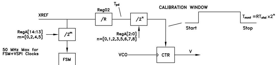
Figure 35. VCO Calibration
