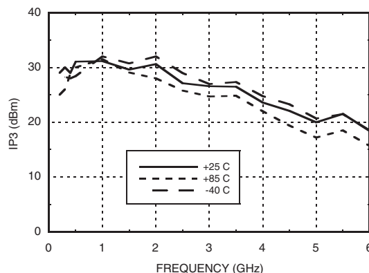
Output IP3 vs. Temperature ( V_{ctl} = 0V ) [1]
