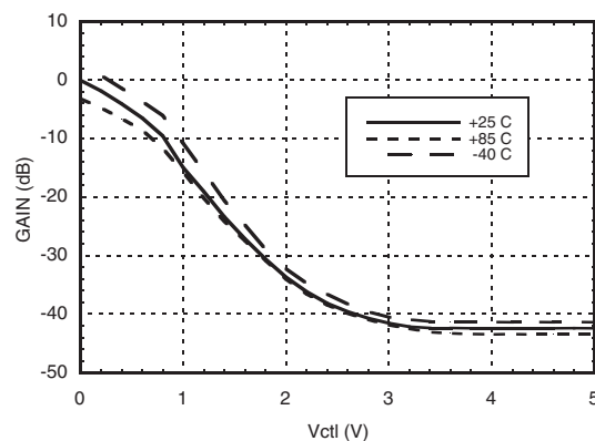
Gain vs. Vctl Over Temperature @ 6 GHz [1]
