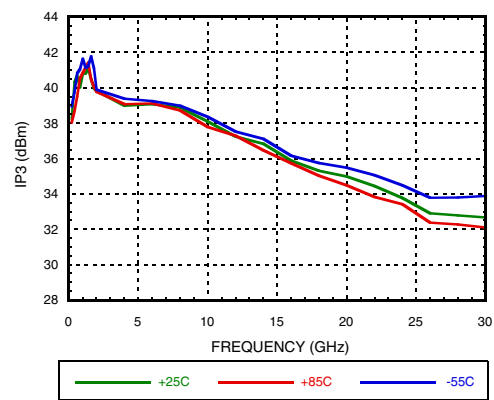
Output IP3 vs. Temperature @ Pout = 16 dBm / Tone
