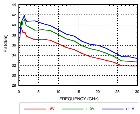
Output IP3 vs. Supply Voltage @ Pout = 16 dBm / Tone
