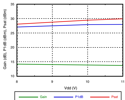
Gain & Power vs. Supply Voltage @ 16 GHz
