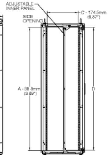
Side View Cross Section
