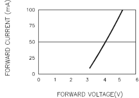
Fig.4 PEAK FORWARD VOLTAGE VS. FORWARD (100us TEST PULSE, 1% DUTY CYCLE)
