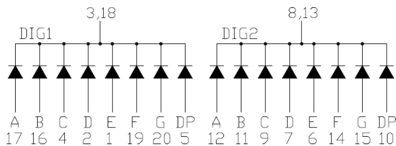
Common Cathode
