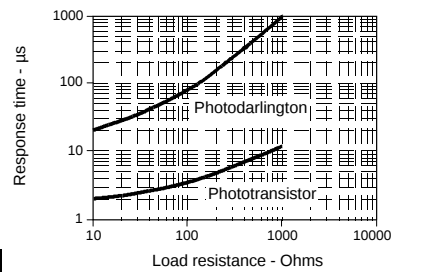
Fig. 2 Non-Saturated Switching Time vs Load Resistance
