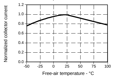
Fig. 4 Collector Current vs Ambient Temperature
