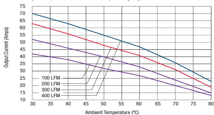
HPH-3.3/70-D48 Maximum Current Temperature Derating ( V_{IN}=48V , Airflow is from V_{IN} to V_{OUT} , no baseplate)
