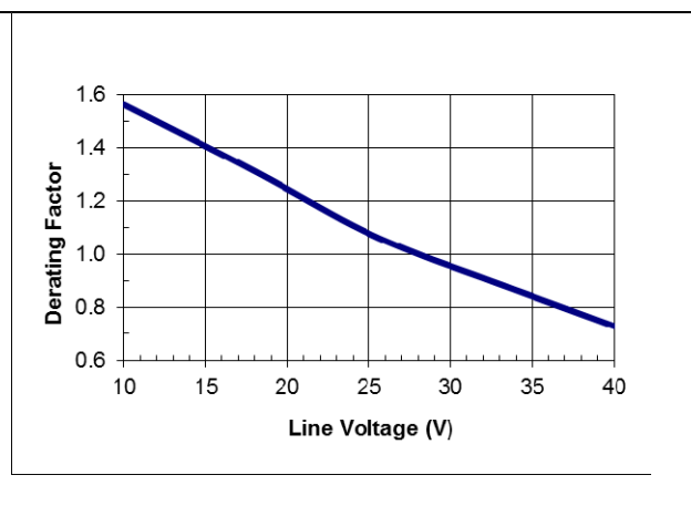
HQA2W120W240V typical temperature derating versus input voltage output with 2m/s (400 lfm) airflow from pin 3 to pin 1.
