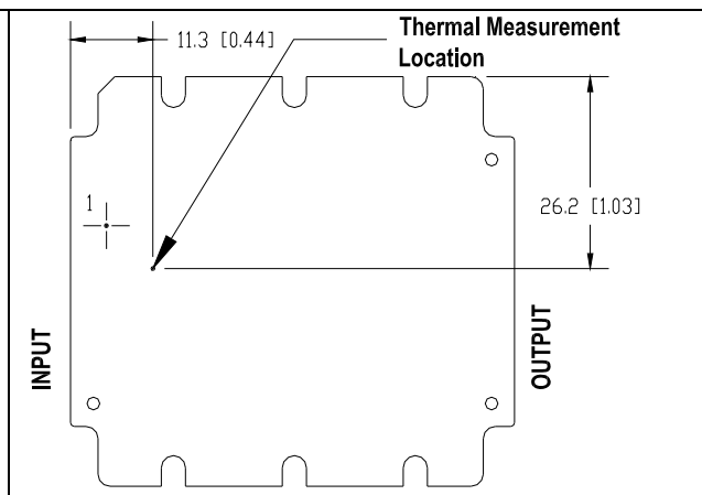
HQA24120W480V-007 thermal measurement location – top view
