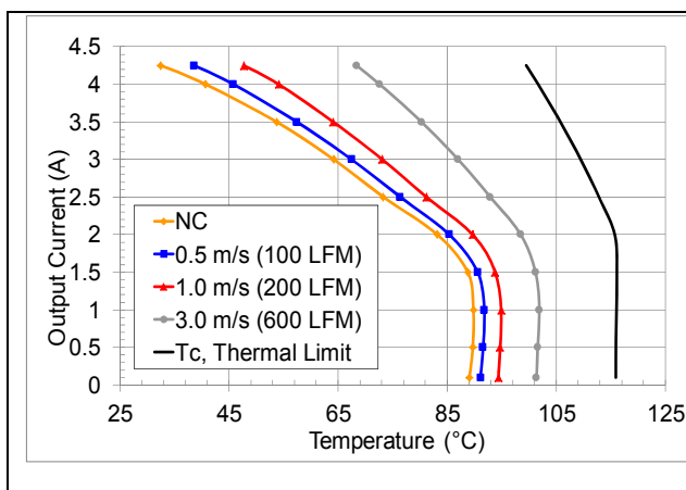
HQA2W120W280V maximum output current vs. ambient temperature at 28V input for airflow rates natural convection (60lfm) to 600lfm with airflow from pin 3 to pin 1
