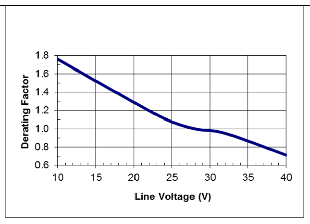
HQA2W120W280V typical temperature derating versus input voltage output with 2m/s (400 lfm) airflow from pin 3 to pin 1.
