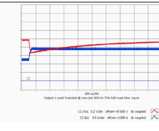
HQA24120W480V Typical transient response. Output voltage response to load step from 50% to 75% of full load with output current slew rate of 0.1A/uS.
