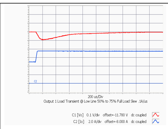
HQA2W120W120V Typical output voltage response to load step from 50% to 75% of full load with output current slew rate of 0.1A/uS and Cext = 500uF
