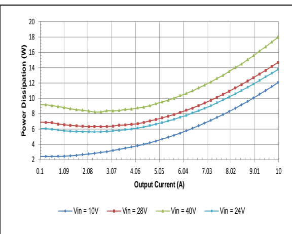
HQA2W120W120V Typical Power Dissipation vs. Input Voltage at Ta=25 degrees
