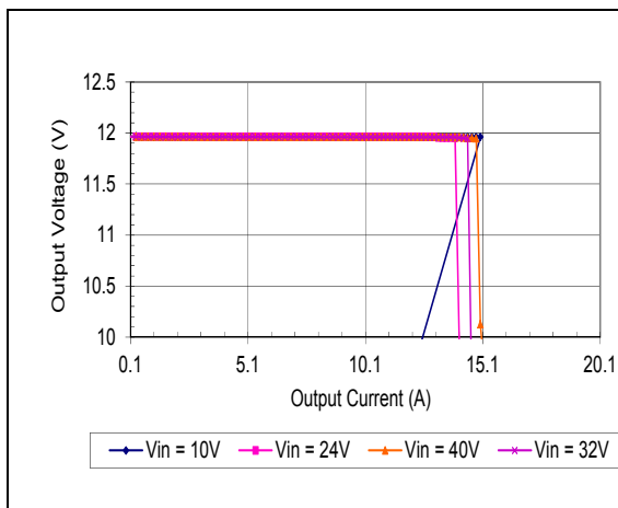
HQA2W120W120V Typical Output Current Limit Characteristics vs. Input Voltage at Ta=25 degrees.
