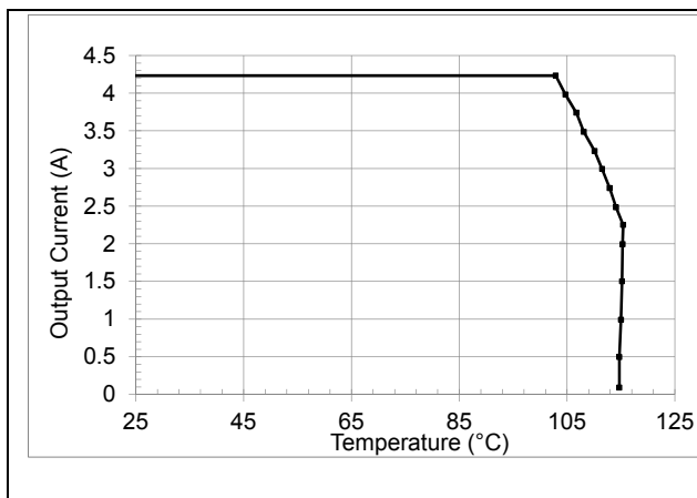
HQA2W120W280V maximum output current vs. baseplate temperature
