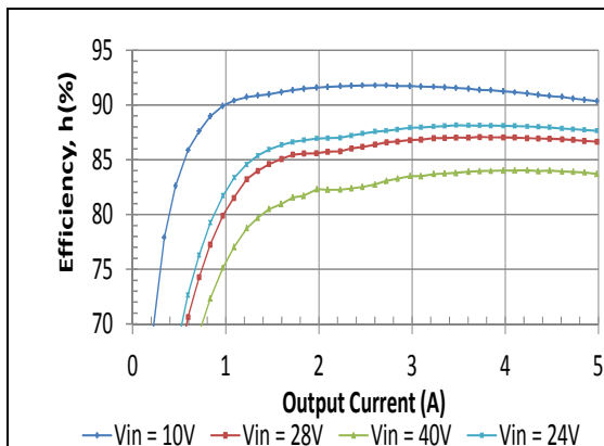
HQA2W120W240V Typical Efficiency vs. Input Voltage at Ta=25 degrees.
