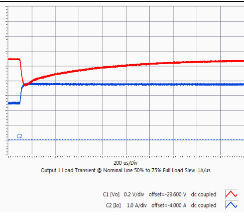
HQA2W120W240V Typical transient response. Output voltage response to load step from 50% to 75% of full load with output current slew rate of 0.1A/uS.
