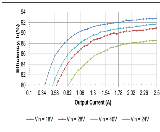
HQA24120W480V Typical Efficiency vs. Input Voltage at Ta=25 degrees.
