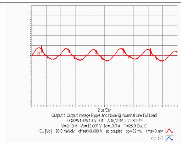
HQA2W120W120V Typical Output Ripple at nominal Input voltage and full load at Ta=25 degree
