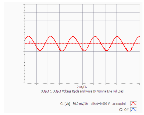
HQA2W120W280V Typical Output Ripple at nominal Input voltage and full load at Ta=25 degree
