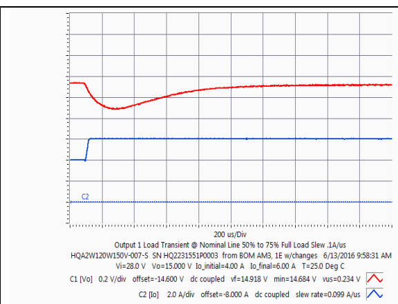
HQA2W120W150V Typical output voltage response to load step from 50% to 75% of full load with output current slew rate of 0.1A/uS and C_{ext} = 500\mu F
