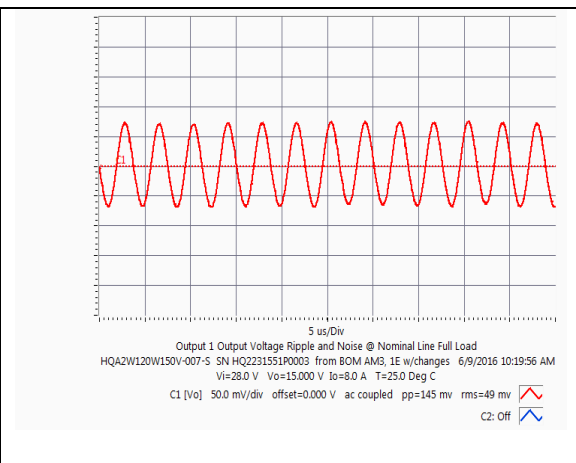
HQA2W120W150V Typical Output Ripple at nominal Input voltage and full load at Ta=25 degree
