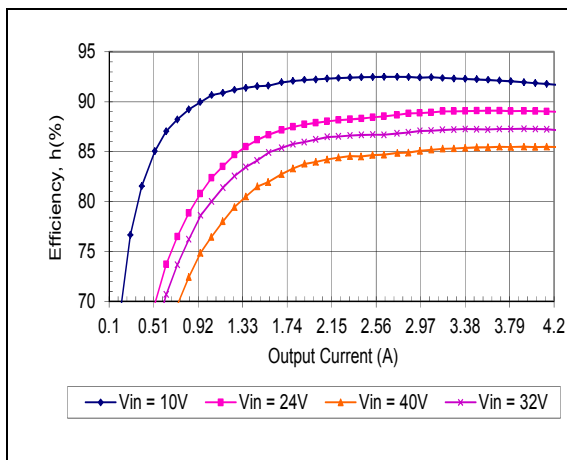
HQA2W120W280V Typical Efficiency vs. Input Voltage at T_a=25 degrees.
