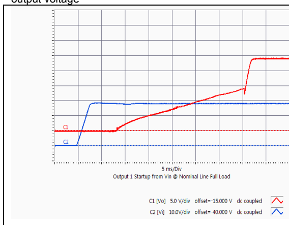
HQA2W120W240V Typical startup characteristic from input voltage application at full load. Red trace - output voltage, blue trace –input voltage
