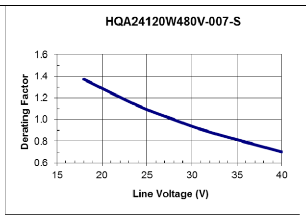
HQA24120W480V typical temperature derating versus input voltage output with 2m/s (400 lfm) airflow from pin 3 to pin 1.
