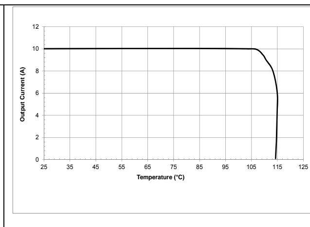
HQA2W120W120V maximum output current vs. baseplate temperature at nominal line
