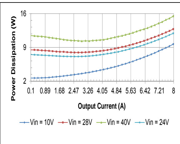
HQA2W120W150V Typical Power Dissipation vs. Input Voltage at T_a=25 degrees
