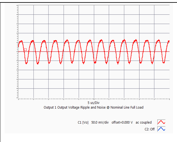
HQA24120W480V Typical Output Ripple at nominal Input voltage and full load at Ta=25 degree
