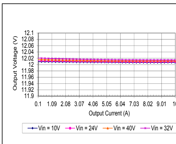
HQA2W120W120V Typical Load Regulation Characteristics at Ta=25 degrees.
