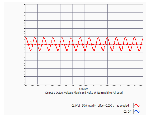
HQA2W120W240V Typical Output Ripple at nominal Input voltage and full load at Ta=25 degree
