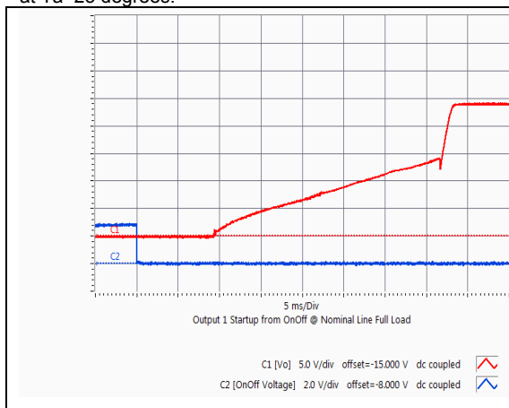
HQA2W120W240V Typical startup characteristic from on/off at full load. Blue trace - on/off signal, red trace – output voltage
