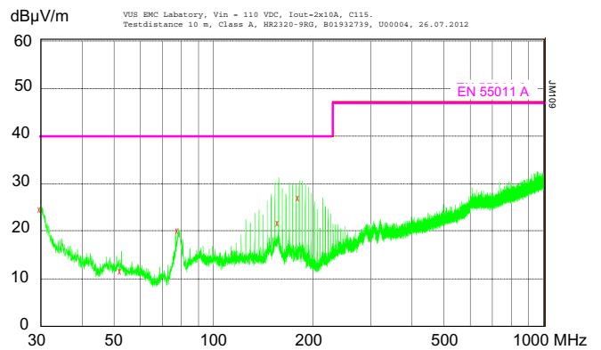
Fig. 17b Typ. radiated emissions accord. to EN 55011/22, antenna 10 m distance, measured at V_i = 110 V and I_{o\text{ nom}} (HR2320-9RG).
