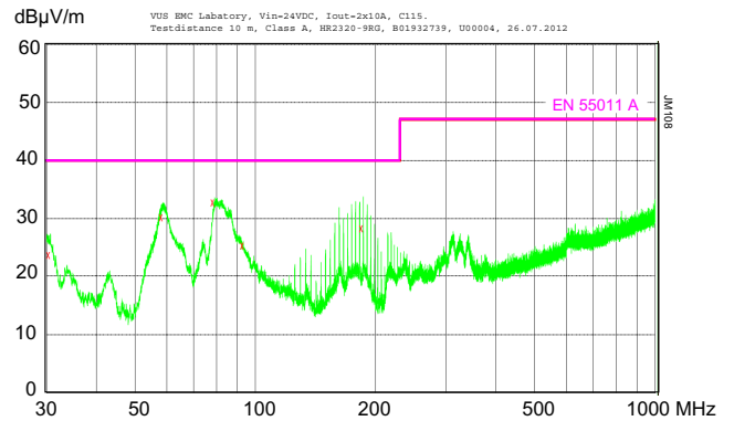
Fig. 17a Typ. radiated emissions accord. to EN 55011/22, antenna 10 m distance, measured at V_i = 24 V and I_{o\text{ nom}} (HR2320-9RG).
