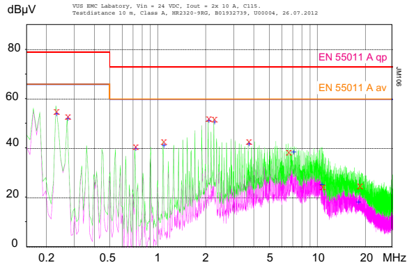
Fig. 16a Typ. conducted emissions (peak/quasipeak and average) at the input according to EN 55011/22, measured at V_i = 24 V and I_{o\text{ nom}} (HR2320-9RG).
