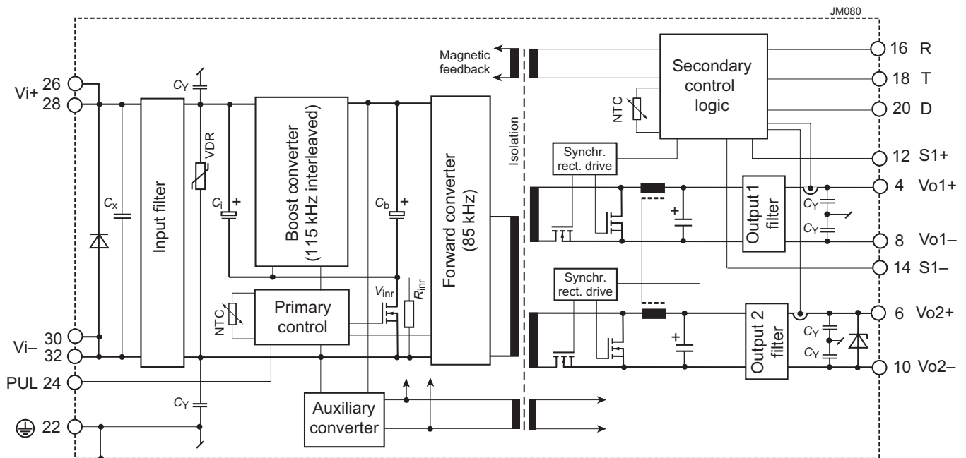
Fig. 1 Block diagram
