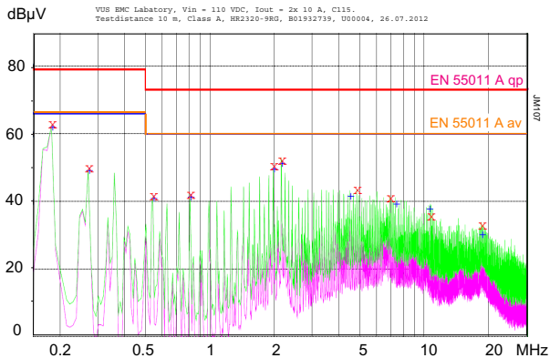
Fig. 16b Typ. conducted emissions (peak/quasipeak and average) at the input according to EN 55011/22, measured at V_i = 110 V and I_{o\text{ nom}} (HR2320-9RG).
