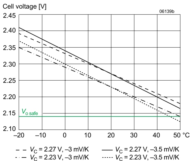
Fig. 15 Trickle charge voltage versus temperature for defined temperature coefficient. V_{o\text{ nom}} is the output voltage with open R-input.
