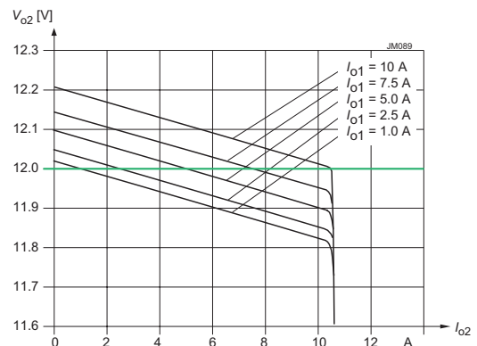
Fig. 11 Models HR2320 (2 outputs 12 V): V_{o2} versus I_{o2} with various I_{o1}
