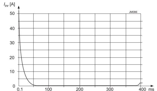
Fig. 5 Inrush current at V_i = 150 V, I_{o nom}
