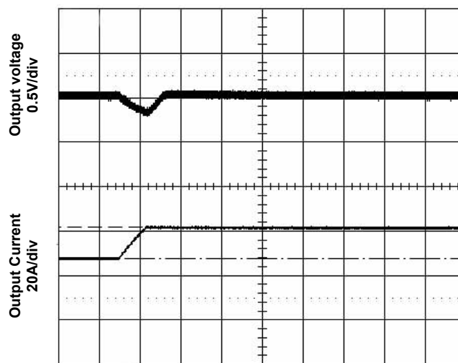
Time - t (200µs/div) Figure 8. Transient Load Response Top: Output voltage deviation Bottom: Load current step (+25% full load) Test Cond.: Output current 27.5A (50% full load), Input voltage 48V, Slew rate 0.1A/µs
