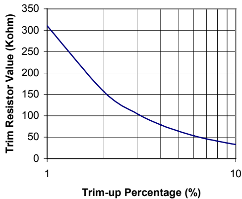
Fig. 19 Trim-Up Resistor Selection
