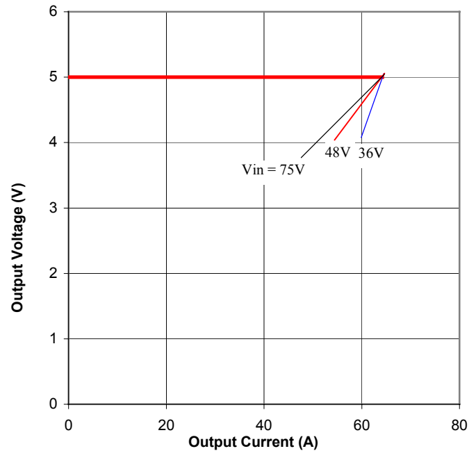
Figure 10. Output Characteristics
