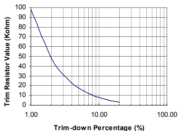
Fig. 18 Trim-Down Resistor Selection
