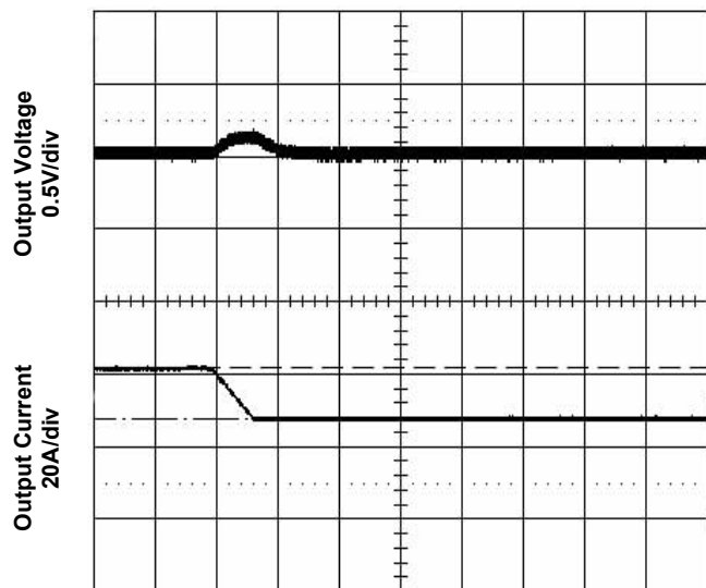
Time - t (200µs/div) Figure 7. Transient Load Response Top: Output voltage deviation Bottom: Load current step (-25% full load) Test Cond.: Output current 27.5A (50% full load), Input voltage 48V, Slew rate 0.1A/µs
