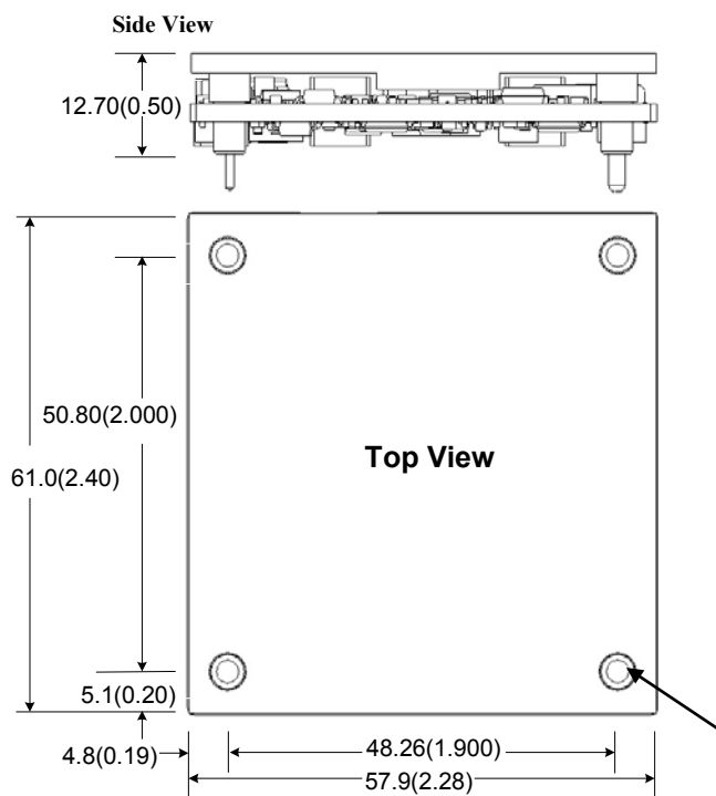
Figure 25. Converter with Optional Baseplate
