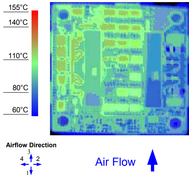
Figure 12. Thermal Image for Airflow Direction 3 (34A output, 55 ^{\circ}C ambient, 200 LFM, V_{in} = 48V open frame unit using socket interface)
