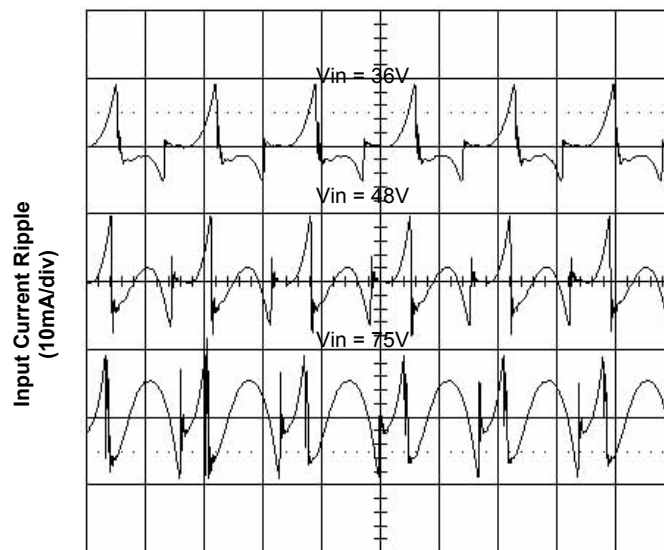
Time - t (2µs/div) Figure 6. Input Reflected Ripple Current at 55A Load
