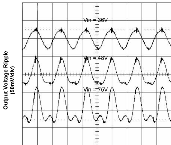
Time - t (2µs/div) Figure 5. Output Ripple Voltage at 55A Load
