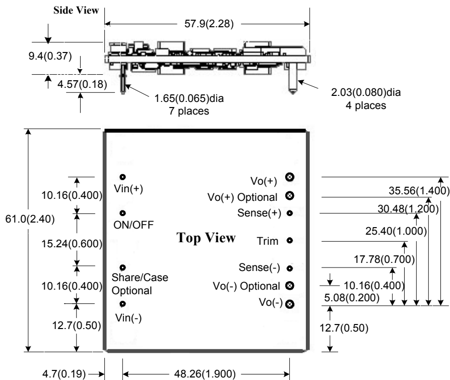
Figure 24. Open Frame Converter
