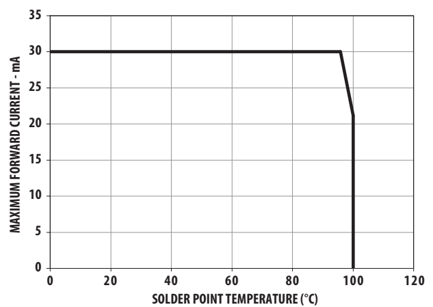
Figure 7d. Maximum Forward Current Vs. Solder Point Temperature. Derated Based on T_{JMAX} = 110^\circ\text{C} , R_{\theta JP} = 110^\circ\text{C/W} (InGaP)
