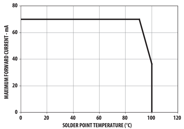
Figure 7b. Maximum Forward Current Vs. Solder Point Temperature. Derated Based on T_{JMAX} = 110^\circ\text{C} , R_{\theta JP} = 110^\circ\text{C/W} (AlInGaP)
