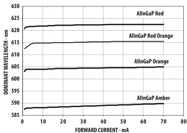
Figure 8a. Dominant Wavelength Vs. Forward Current (AlInGaP)
