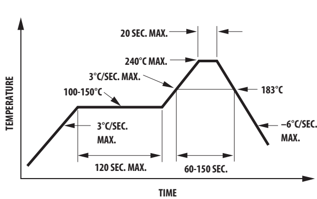
Figure 11a. Recommended SnPb Reflow Soldering Profile.
