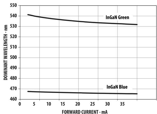
Figure 8b. Dominant Wavelength Vs. Forward Current (InGaP)
