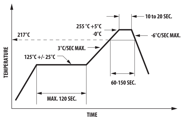
Figure 11b. Recommended Pb-free Reflow Soldering Profile
