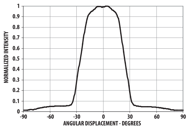
Figure 10. Radiation Pattern
