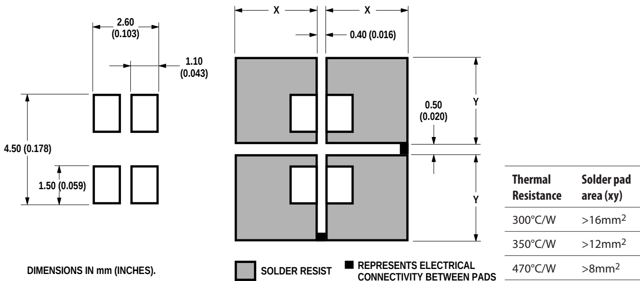
Figure 12. Recommended Soldering Pad Patter
