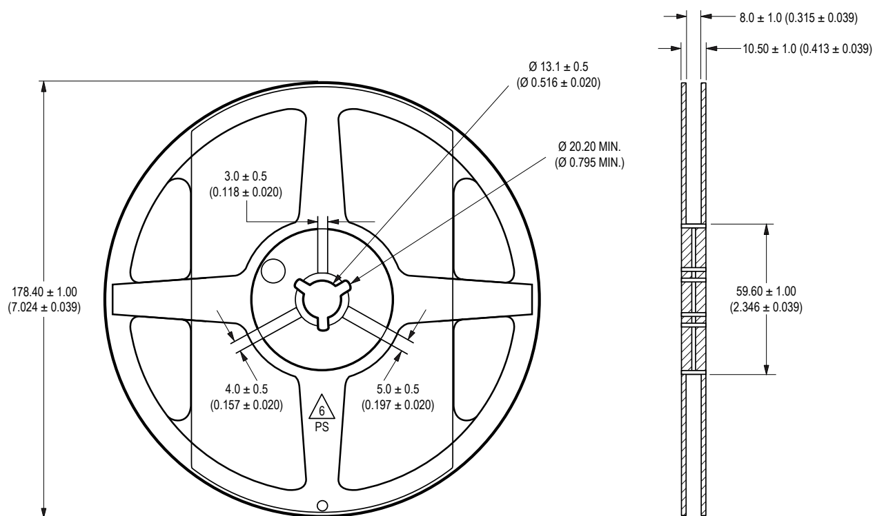
Figure 10. Reel dimensions.
