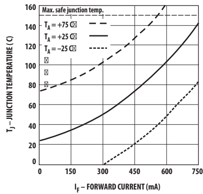
Figure 4. Junction Temperature vs. Current as a Function of Heat Sink Temperature for HSMS-270B and HSMS-270C. Note: Data is calculated from SPICE parameters.
