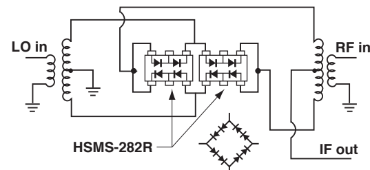
Figure 23. Low Distortion Double Balanced Mixer.
