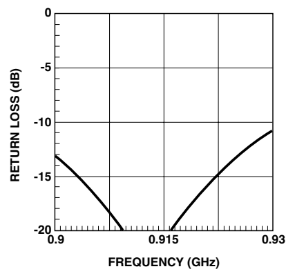
Figure 12. Input Return Loss.
