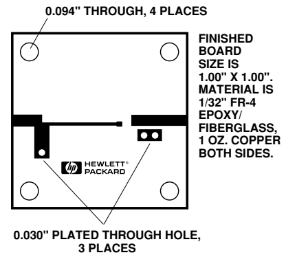
Figure 15. Physical Realization.
