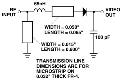
Figure 11. 915 MHz Matching Network for the HSMS-286x Series at 3 µA Bias.
