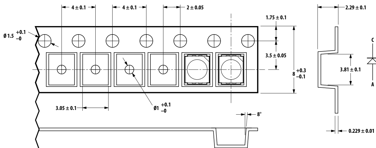
Figure 12. Tape dimensions
