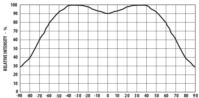
Figure 9. Relative intensity vs. angle for HSMW-C265.
