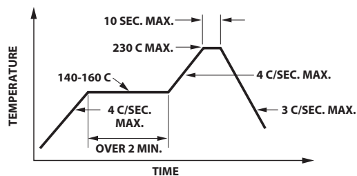
Figure 10. Recommended reflow soldering profile.
