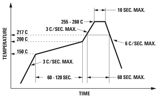
Figure 11. Recommended Pb-free reflow soldering profile.
