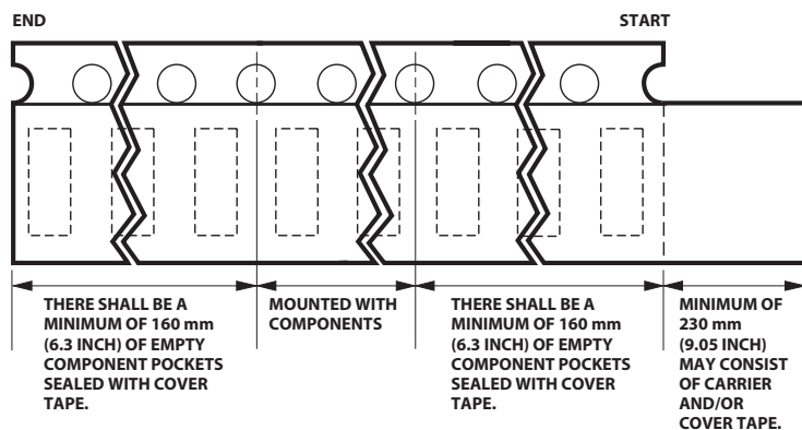
Figure 18. Tape leader and trailer dimensions.
