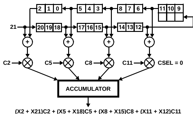
FIGURE 17A. COMPUTATIONAL FLOW AS DATA SAMPLE 21 IS CLOCKED INTO THE FEED-FORWARD STAGE
