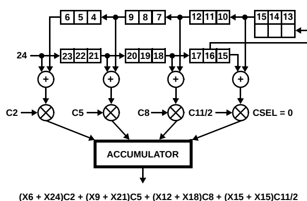
FIGURE 20D. COMPUTATIONAL FLOW AS DATA SAMPLE 24 IS CLOCKED INTO THE FEED-FORWARD STAGE TXFR TAKES AFFECT ON THIS CLOCK CYCLE
