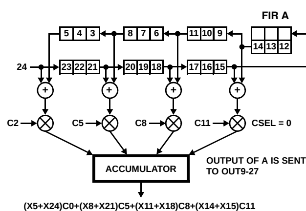
FIGURE 26D. COMPUTATIONAL FLOW AS DATA SAMPLE 24 IS CLOCKED INTO THE FEED-FORWARD STAGE
