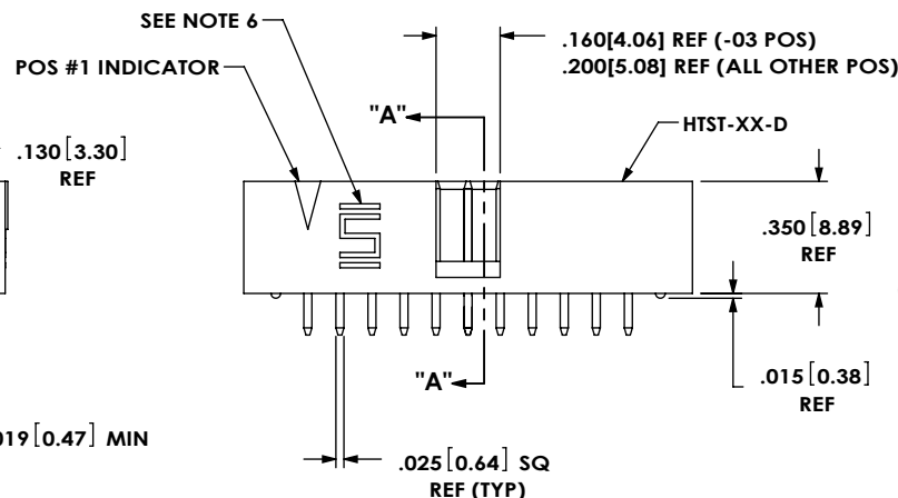
FIG 1 HTST-111-01-XX-D-LL SHOWN * DIMENSIONS APPLY WHEN USING -LL OPTION ONLY
