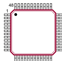
48-Lead LQFP (FG) (top view)
