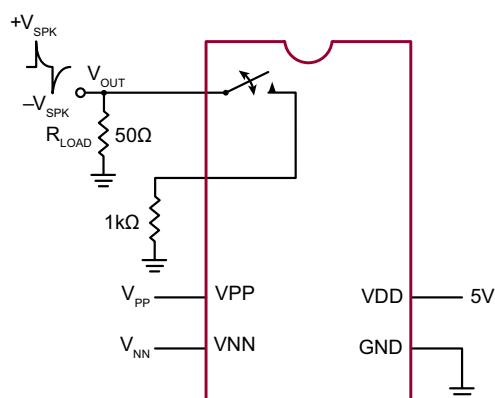
Output Voltage Spike
