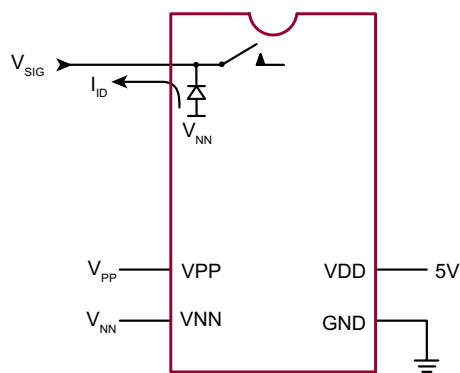
Output Switch Isolation Diode Current
