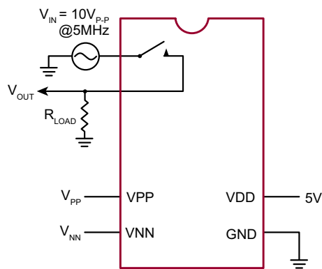
K_O = 20 \log \frac{V_{OUT}}{V_{IN}} OFF Isolation
