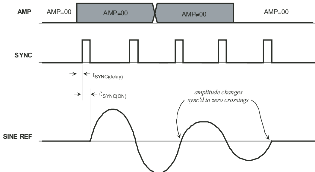
Figure 4: AMP Timing
