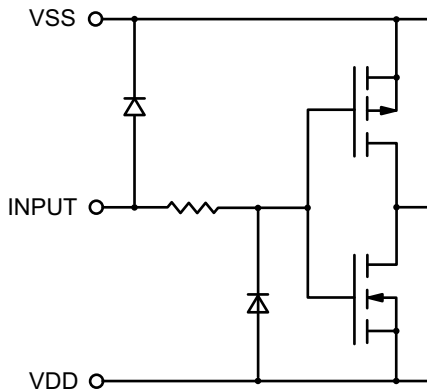
Logic Inputs
