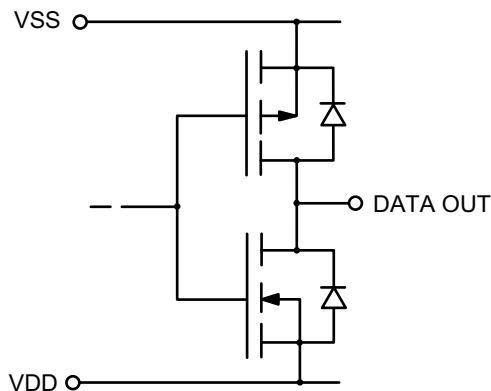
Logic Data Output
