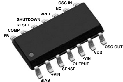
14-Lead Narrow Body SOIC (NG)
