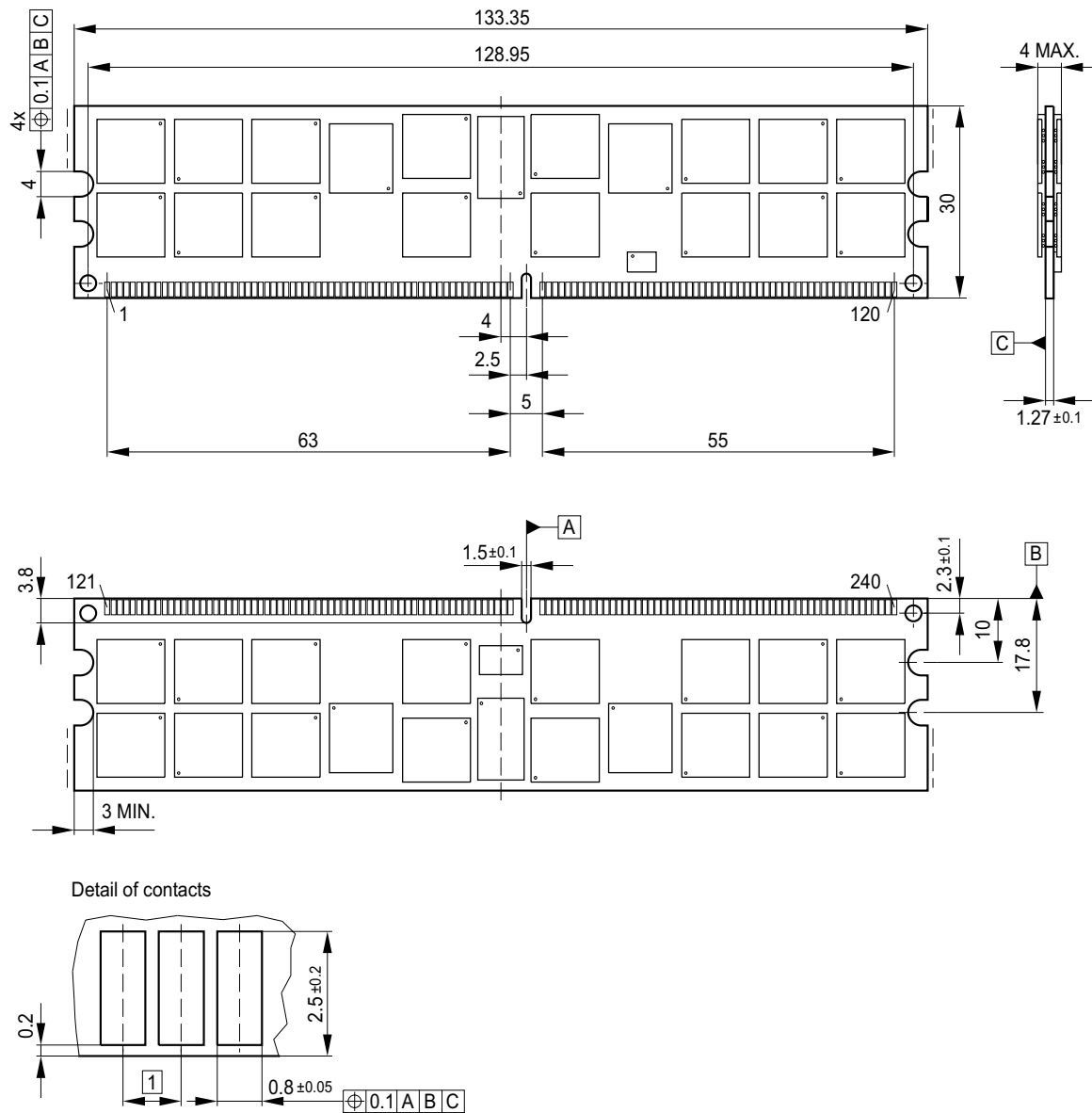
FIGURE 9 Package Outline Raw Card L L-DIM-240-40
