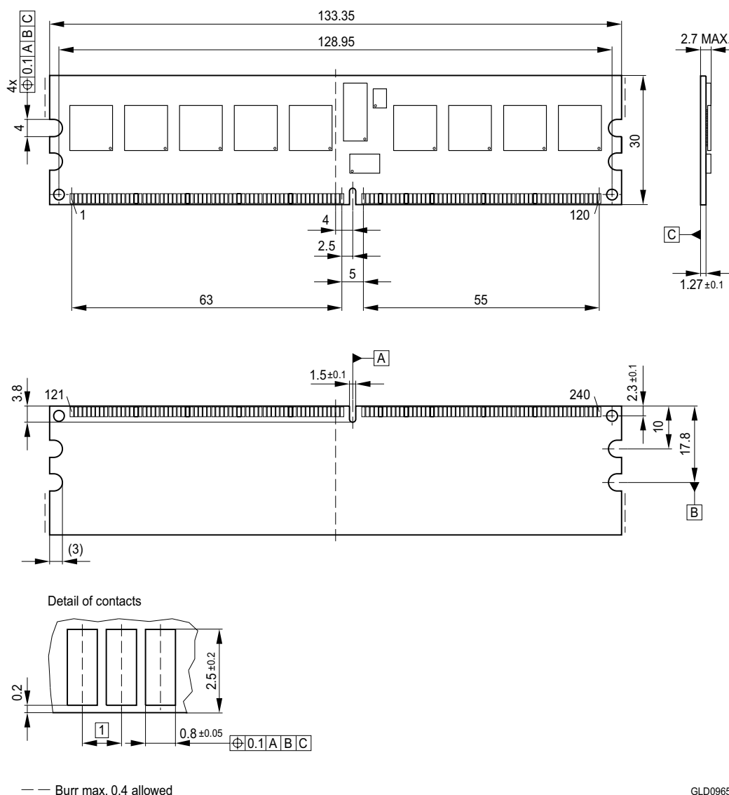
FIGURE 5 Package Outline Raw Card A L-DIM-240-11
