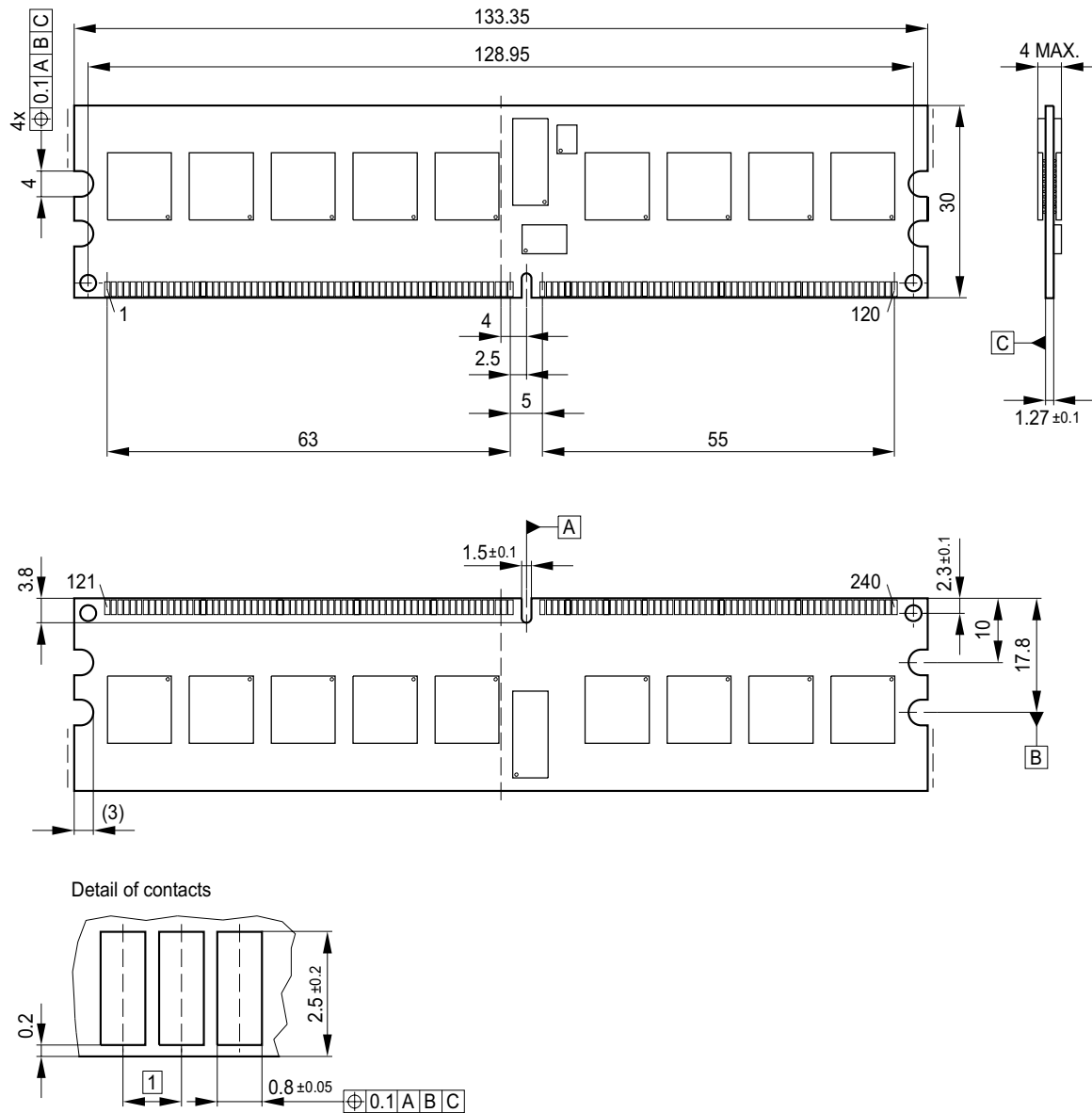
FIGURE 6 Package Outline Raw Card B-G L-DIM-240-12
