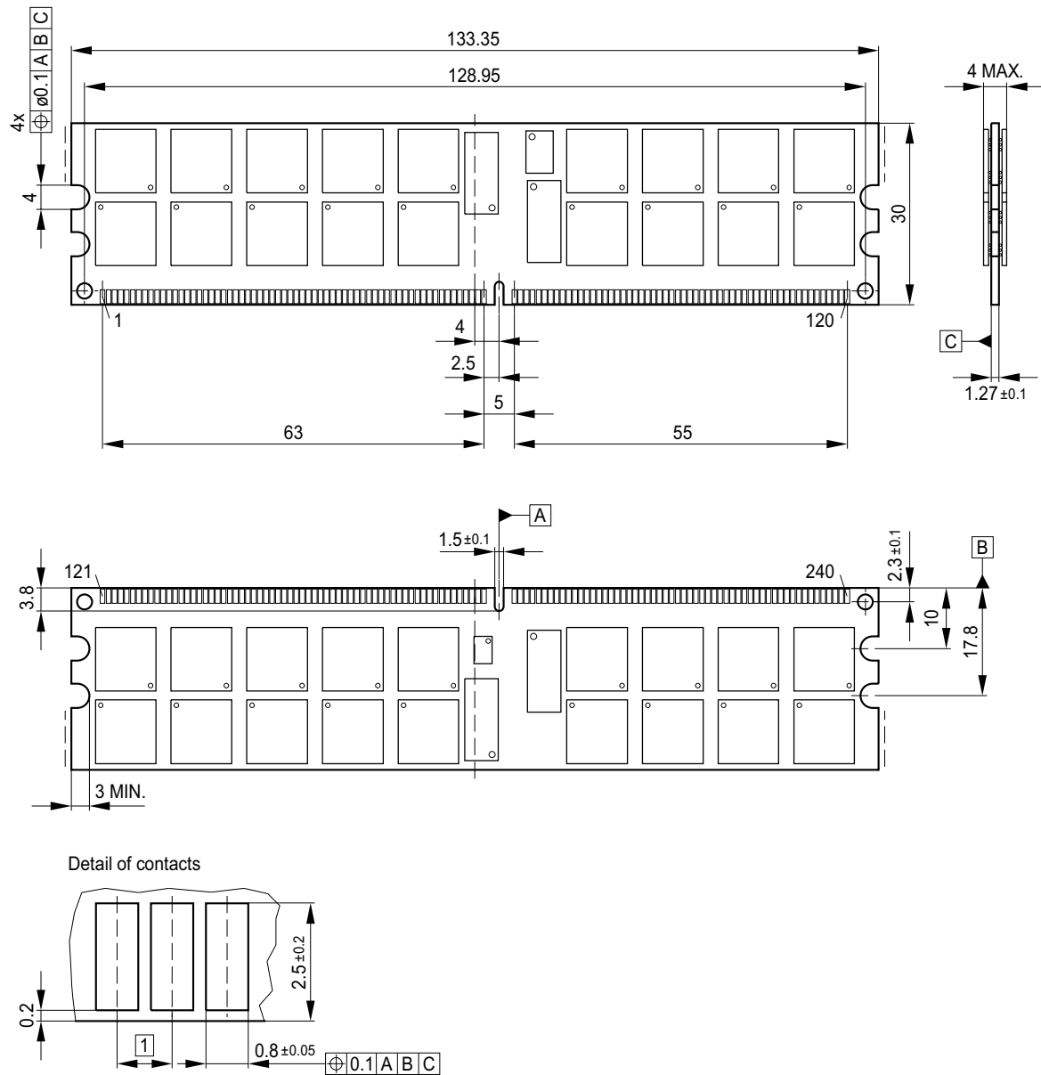
FIGURE 10 Package Outline Raw Card N – L-DIM-240-44
