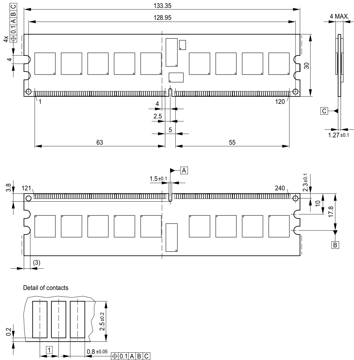
FIGURE 7 Package Outline Raw Card C L-DIM-240-13
