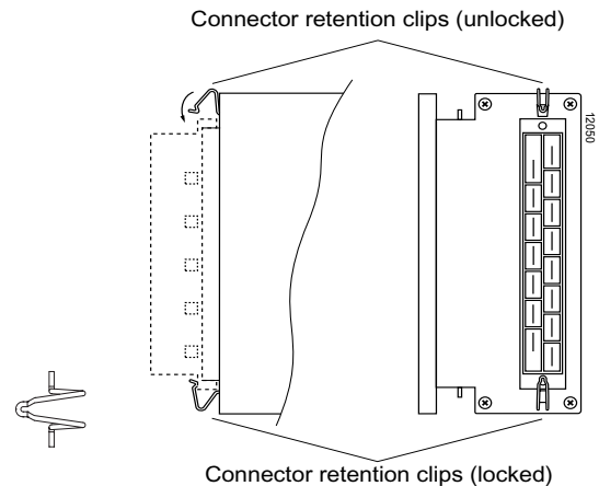
Fig. 19 Connector retention clips HZZ01209-G and their application
