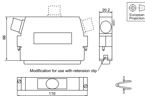
Fig. 22 Cable hood HZZ00142-G for fastening with retention clips HZZ01209-G
