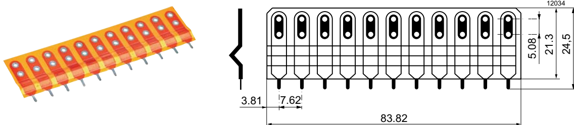
Fig. 6 Flexible H11 flexible PCB board HZZ01208-G
