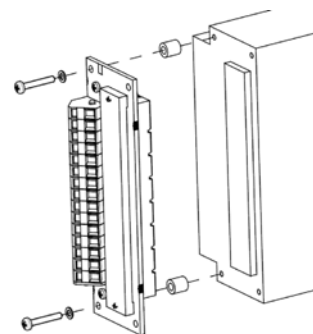
Fig. 24 Cage clamp adapter HZZ00144-G
