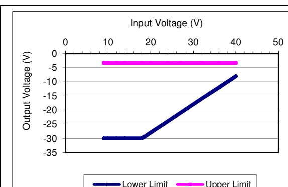
Output Voltage versus Input Voltage Operating Range
