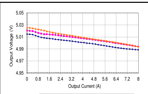
Vo=-5V Typical load regulation
