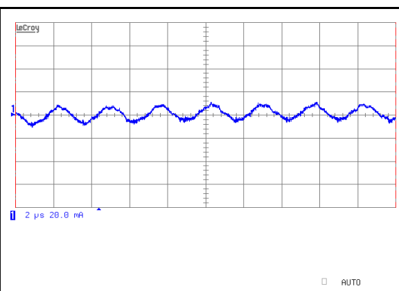
Vo=-12V Typical Input Ripple at nominal Input Voltage and full load at Ta=25 degrees. Input capacitors 1x 22uF ceramic and 1x100uF electrolytic
