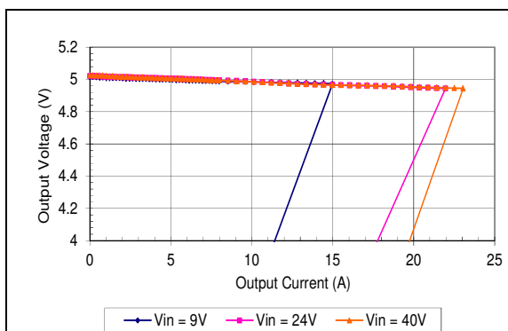
Vo=-5V Typical Current Limit Characteristics
