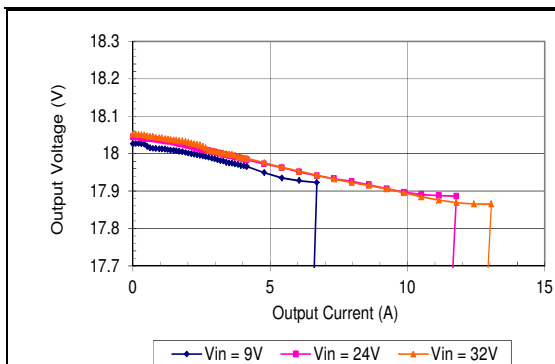
Vo=-18V Typical Current Limit Characteristics
