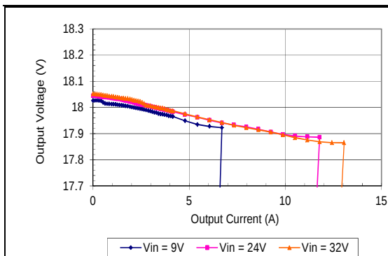
V_o = -18V Typical Current Limit Characteristics
