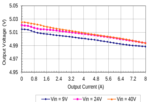
V_o = -5V Typical load regulation
