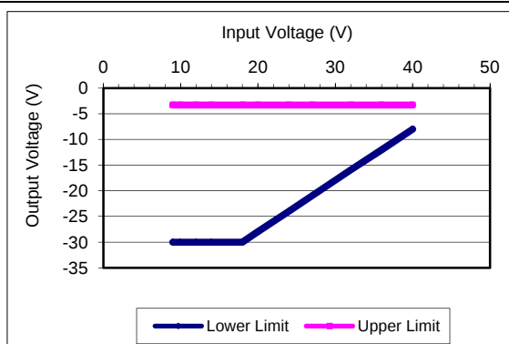
Output Voltage versus Input Voltage Operating Range
