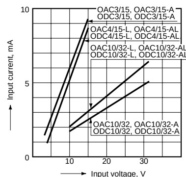
3. Input current vs. input voltage characteristics (OAC, ODC)
