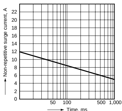
2-2. Non-repetitive surge current vs. time characteristics (ODC)
