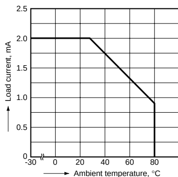
1-1. Load current vs. ambient temperature characteristics (OAC)
