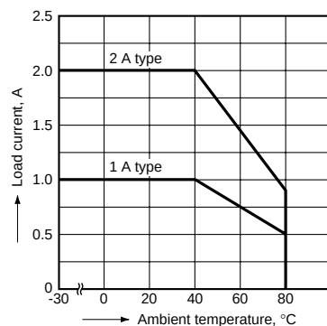
1-2. Load current vs. ambient temperature characteristics (ODC)
