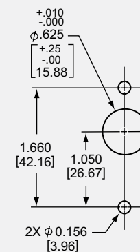
Single Pole Mounting Detail
