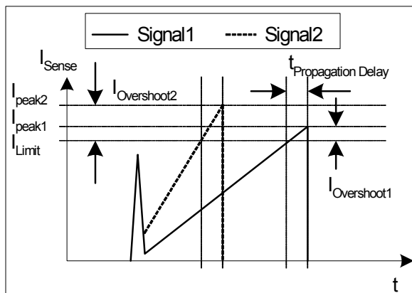
Figure 17 Current Limiting
