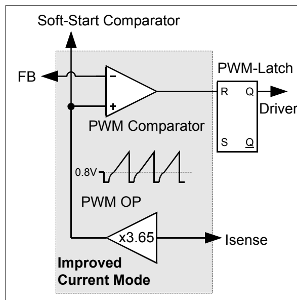
Figure 7 Current Mode
