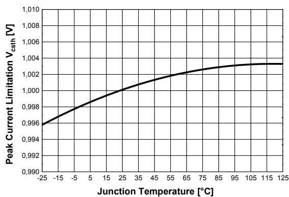
Figure 49 Peak Current Limitation V_{csth} vs. T_j
