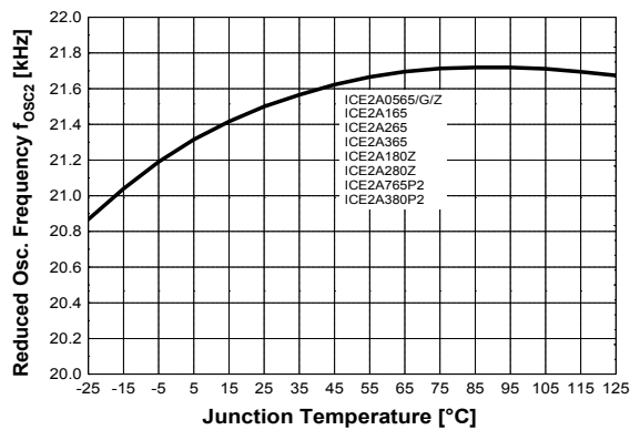
Figure 37 Reduced Osc. Frequency f_{OSC2} vs. T_j
