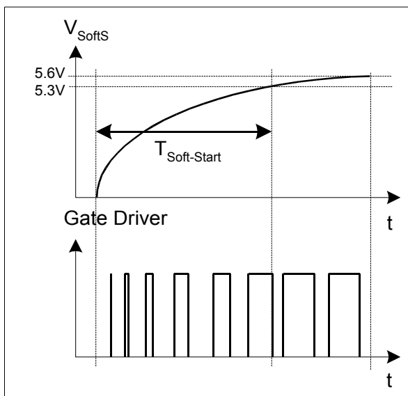
Figure 12 Soft-Start Phase
