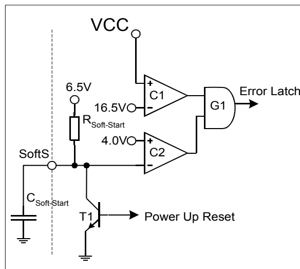
Figure 24 Overvoltage Detection
