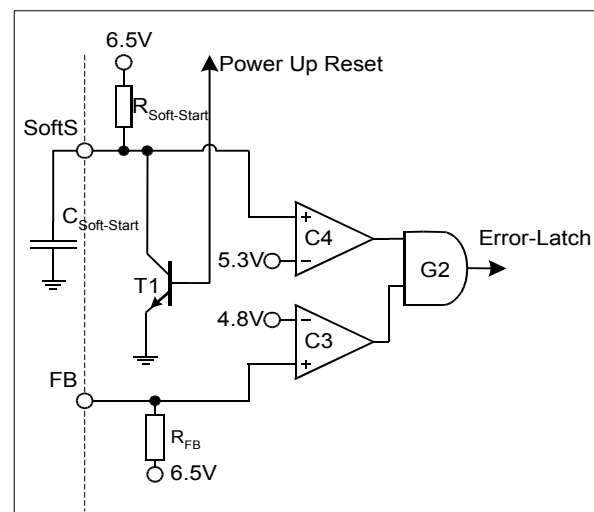
Figure 22 FB-Detection
