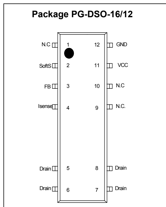
Figure 4 Pin Configuration PG-DSO-16/12 (top view)
