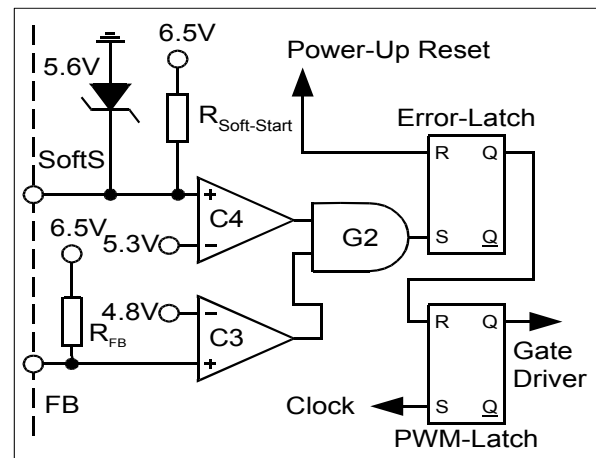
Figure 13 Activation of Protection Unit
