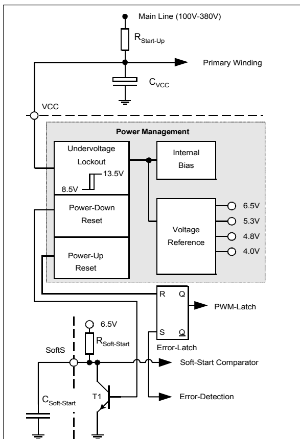
Figure 6 Power Management
