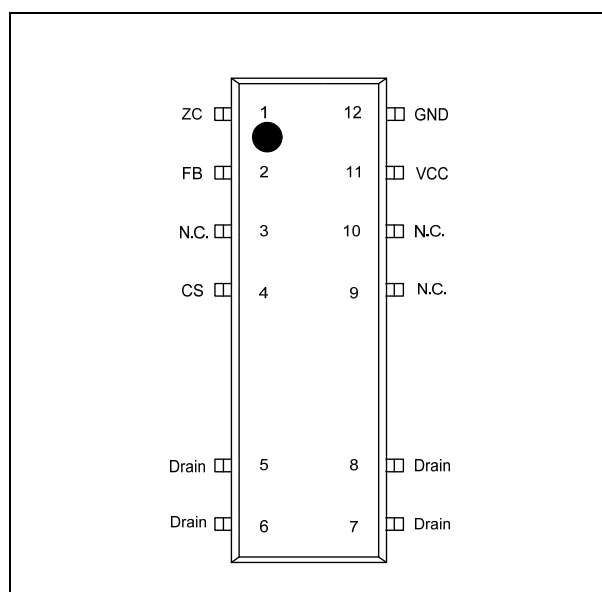
Figure 2 Pin configuration PG-DSO-16/12 (top view)
