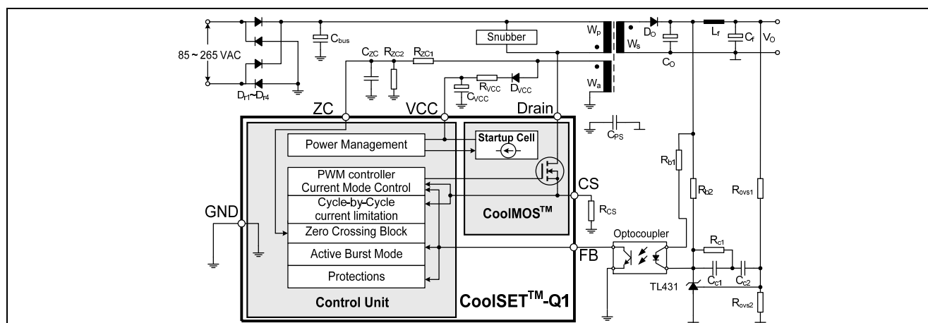
Figure 1 Typical Application
