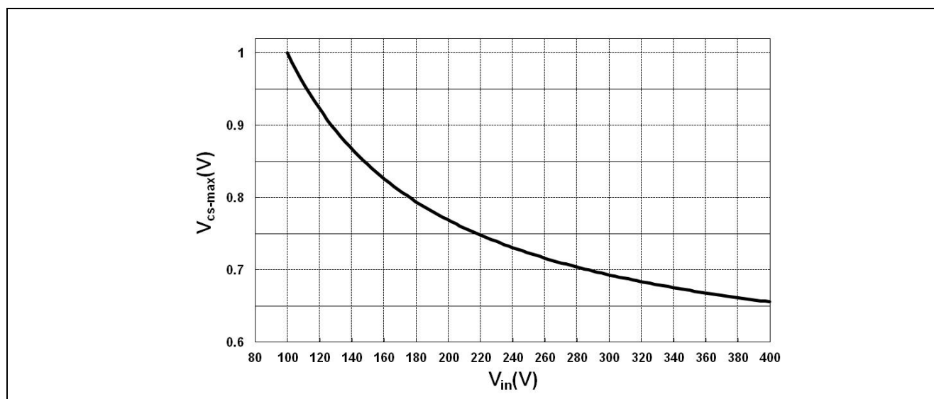
Figure 7 Variation of the V_{CS} limit voltage according to the I_{ZC} current
