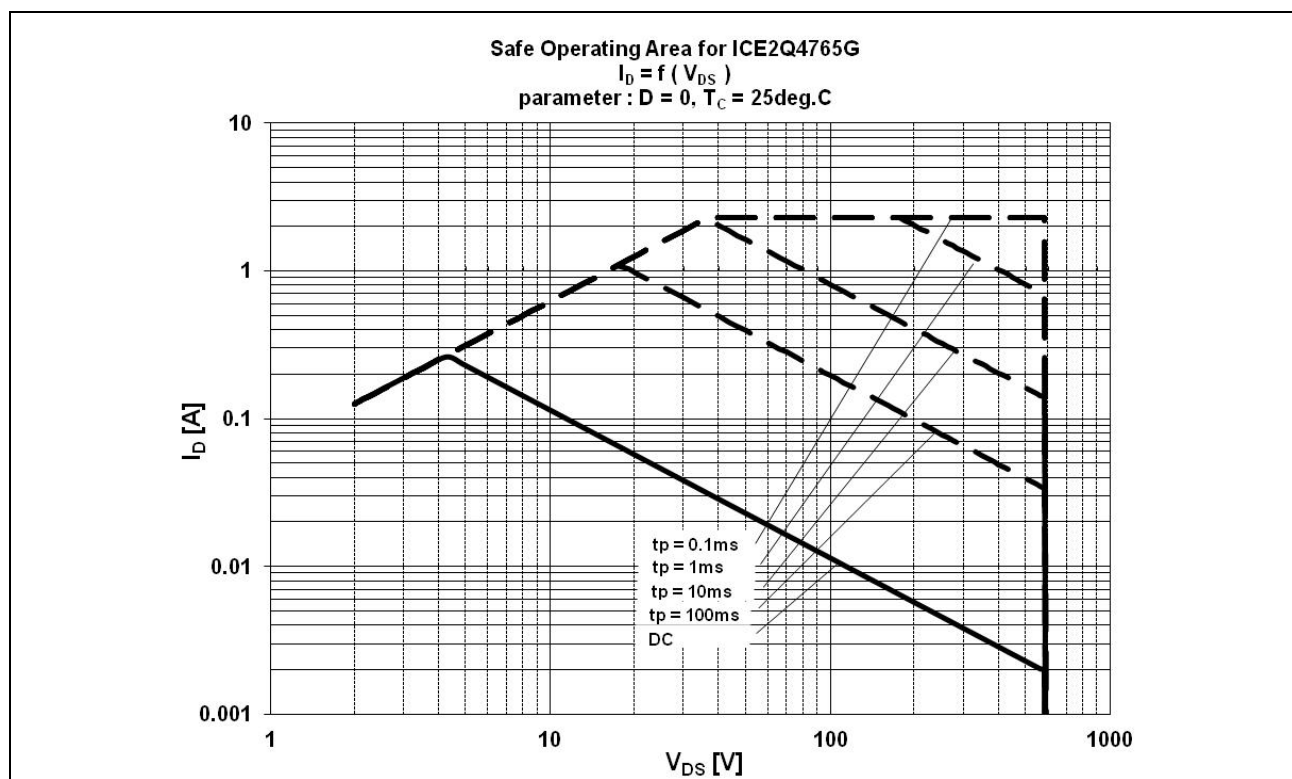
Figure 10 Safe Operating Area (SOA) curve for ICE2QR4765G
