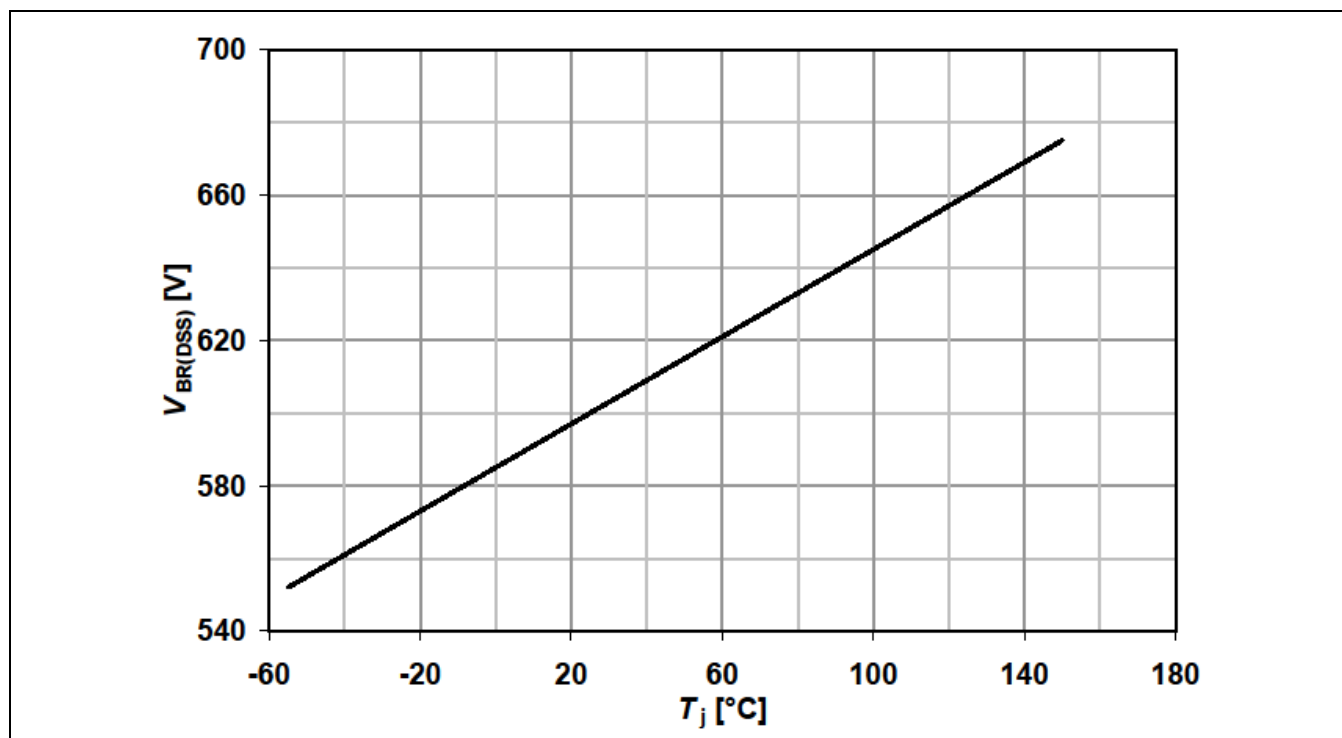
Figure 12 Drain-source breakdown voltage; V_{BR(DSS)}=f(T_j)
