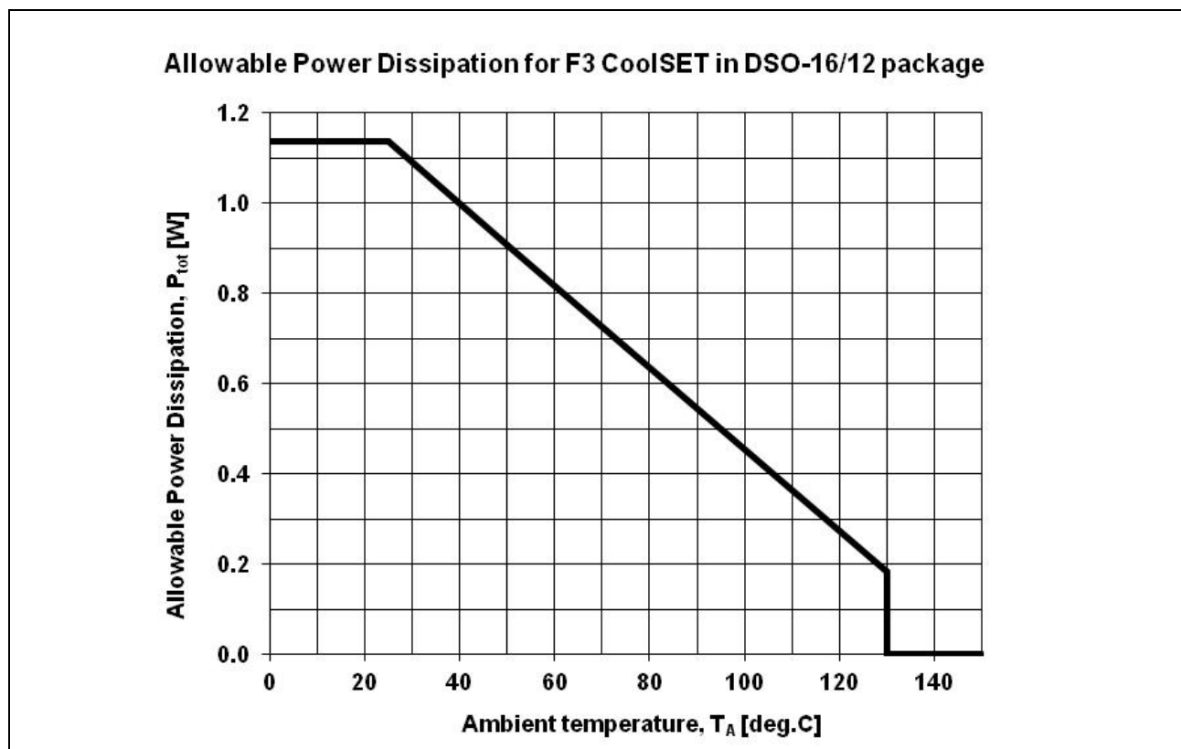
Figure 11 Power dissipation; P_{tot}=f(T_A)
