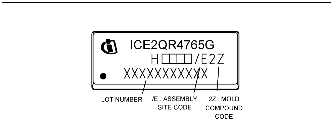
Figure 16 Marking for ICE2QR4765G
