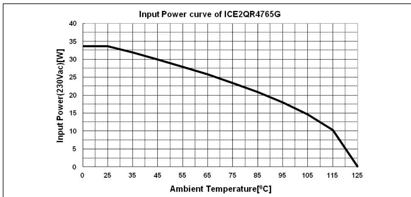
Figure 14 Input Power curve V_{in}=230V_{ac} ; P_{in}=f(T_a)
