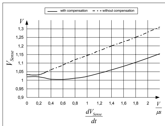
Figure 20 Overcurrent Shutdown
