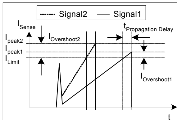
Figure 19 Current Limiting
