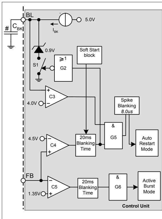
Figure 22 Basic and Extendable Blanking Mode
