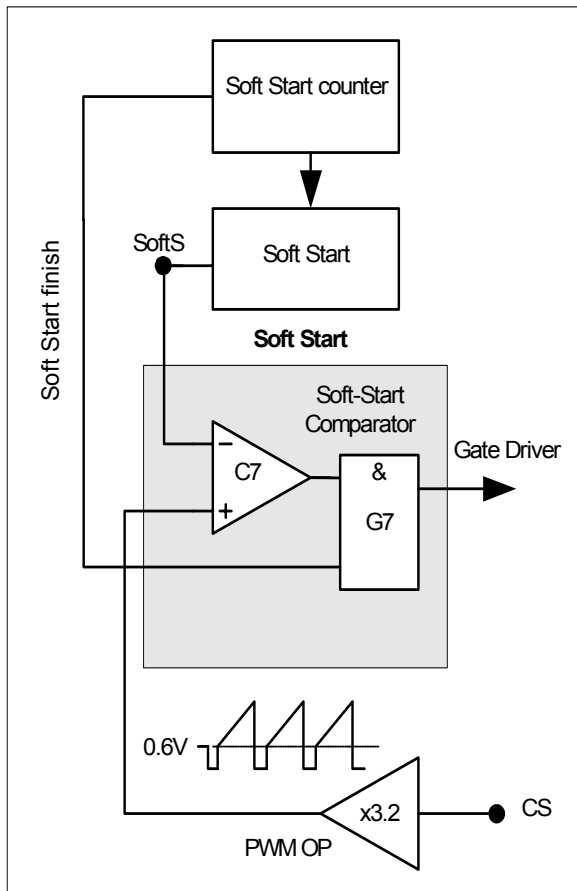
Figure 9 Soft Start
